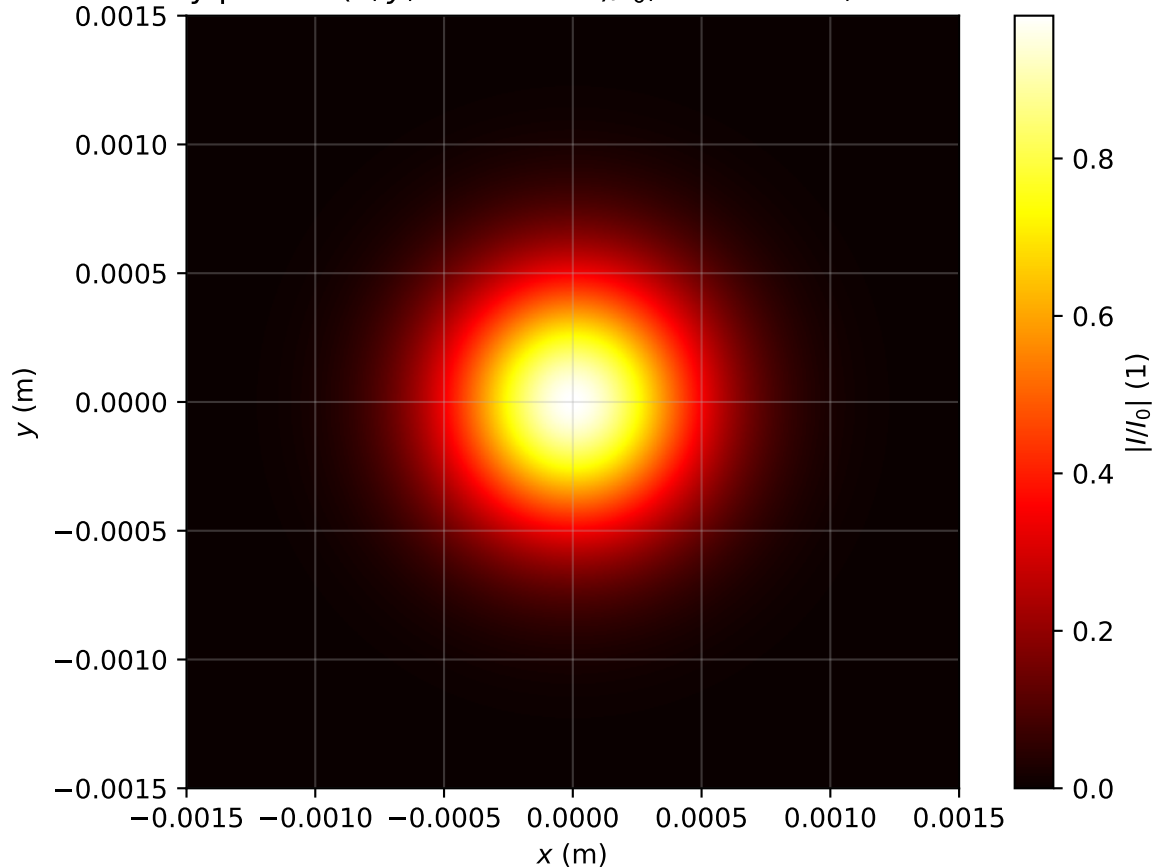
Intensity profile I(x, y, z = 0.716m)/I_0 , Pin=0.3Pcr, artificial time
